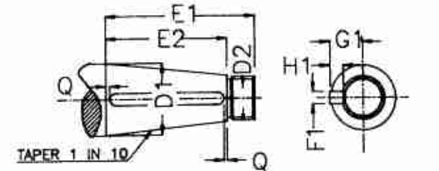
TAPERED SHAFT DETAILS (BOTH ENDS IDENTICAL) KEY IS PARALLEL TO THE SHAFT AXIS
